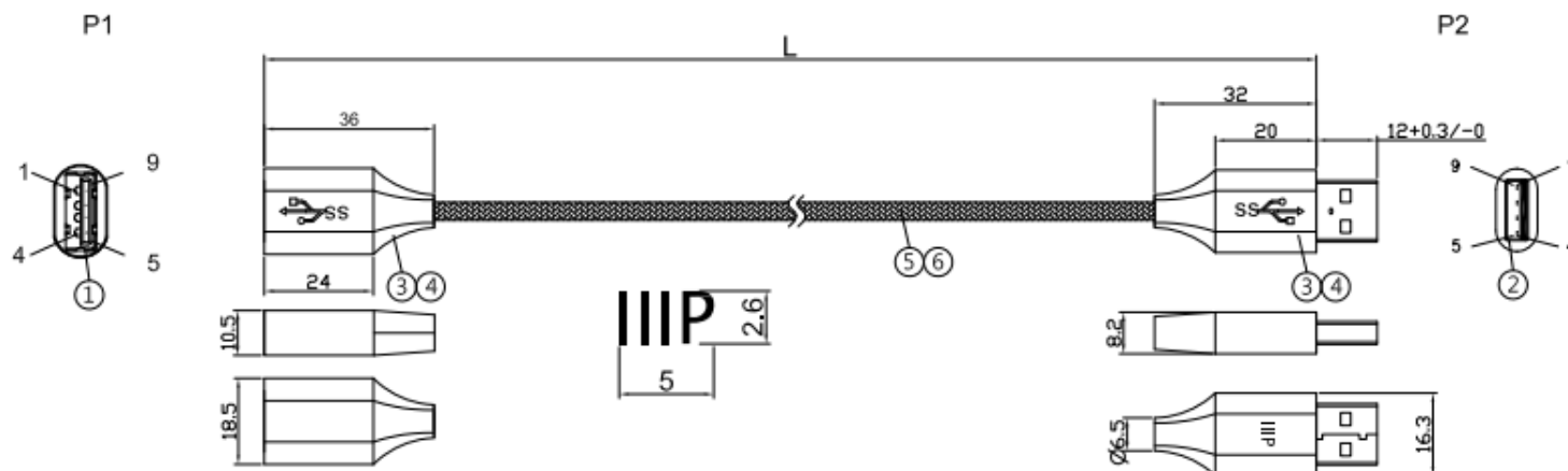
USB 3.0(A)/F MOLDING TYPE
